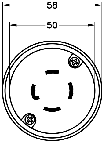
NEMA L16-30 PLUG FRONT VIEW
